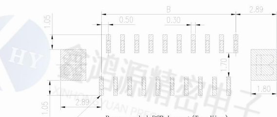
Recommended PCB Layout (Top View) Recommended metal mask pattern (Thickness 0.1mm)
