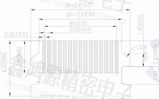
APPLICABLE FPC/FFC (THICKNESS 0.3±0.03)
