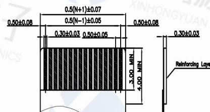
RECOMMENDED FFC DIM
