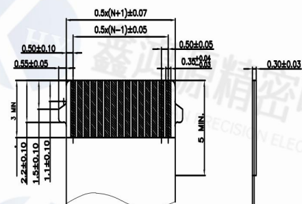
RECOMMENDED FFC DIM
